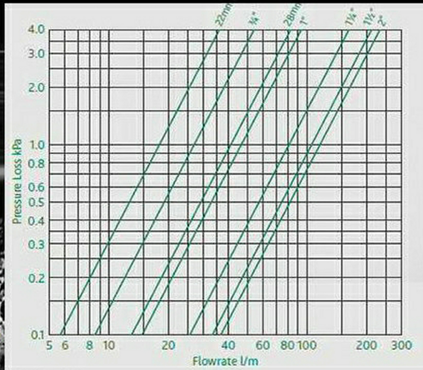
LINEAR RELATIONSHIP BETWEEN PRESSURE LOSS AND FLOWRATE
